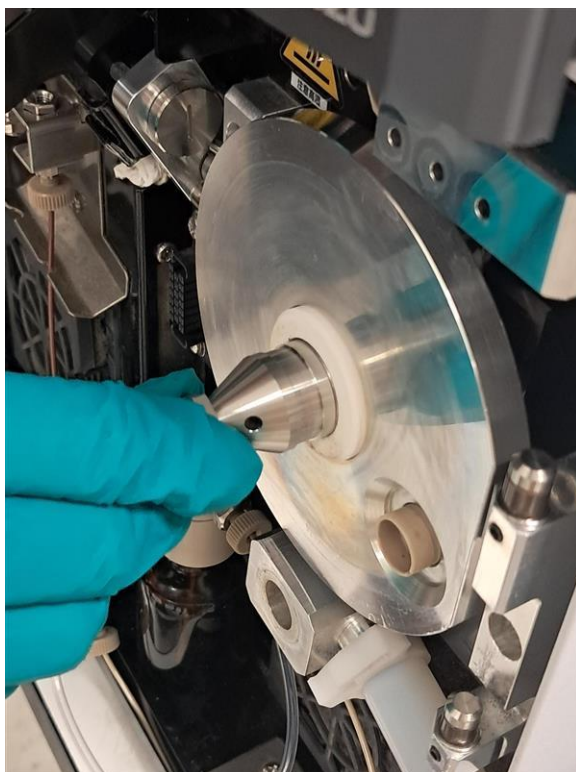
Figure 4 : SICRIT® Ion source adapter mounted on heat block.
