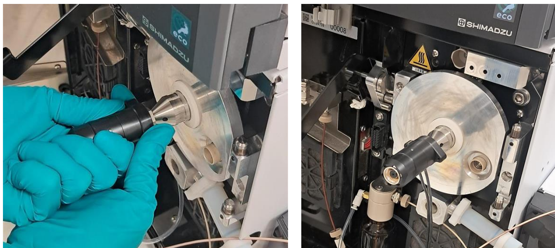
Figure 5: SICRIT® Ion source mounting on the SICRIT Adapter assembly.
