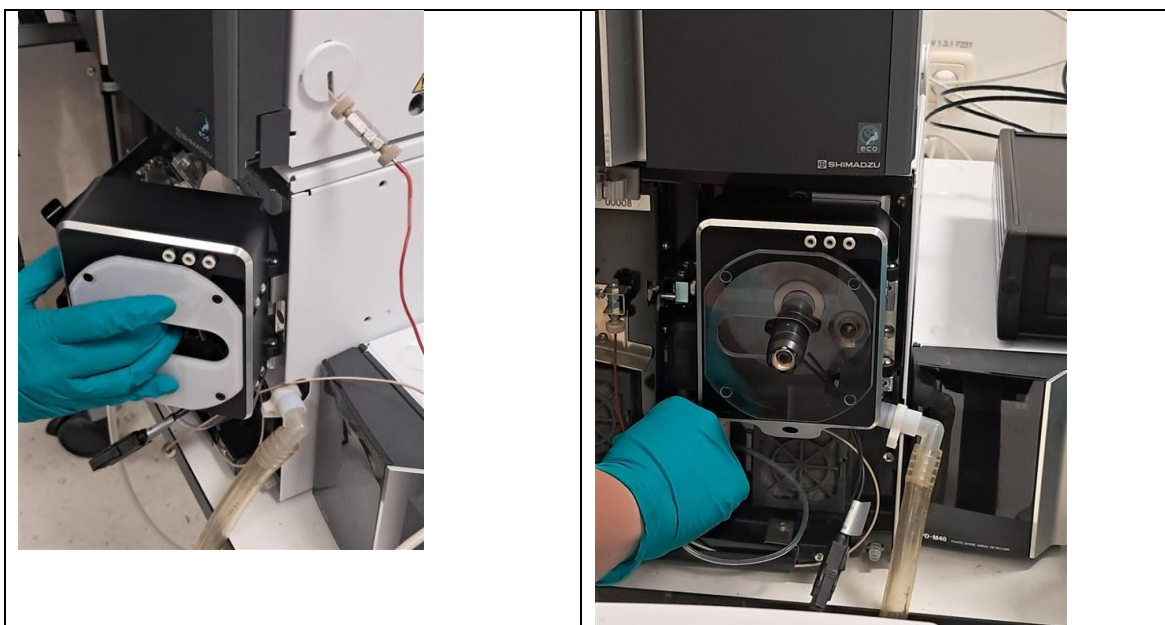
Figure 6: Hooking of SICRIT® Interlock on the MS interface and closing the lock lever.
